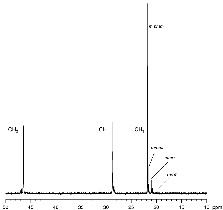
Figure 3. ^{13}\text{C} NMR spectrum ( 1,1,1,2,2\text{-C}_2\text{D}_2\text{Cl}_4 , 125 MHz, 135^\circ\text{C} ) of isotactic polypropylene formed by 12 /MAO at 0^\circ\text{C} . The presence of the unmarked peak in the methyl region is due to regioversions.
